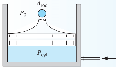
FIGURE 2.11 Sketch for Example 2.3.
