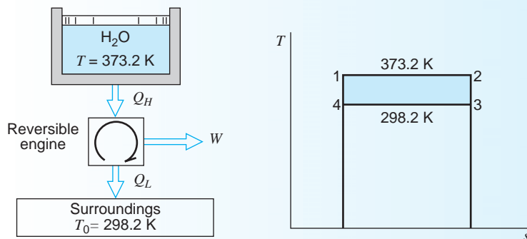
FIGURE 8.20 Reversible heat transfer with the surroundings.
