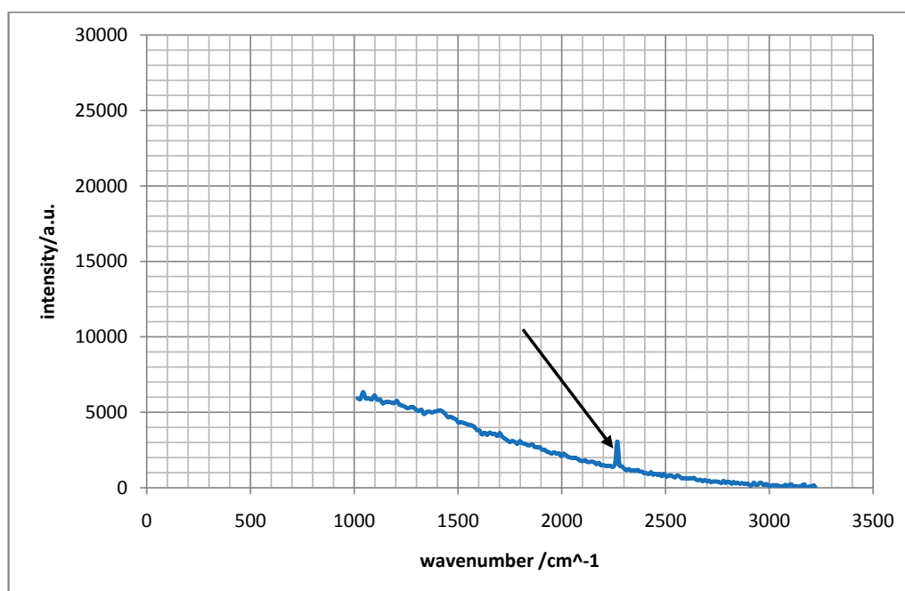
Figure 5.23: Raman-spectra of \text{CHCl}_3 (top) and \text{CDCl}_3 (bottom) showing the isotope effect (see peaks at highest wave number as indicated by arrows). Both spectra were measured with an iRaman-spectrometer by W. Schärtl at university Mainz, Germany, August 2013.
