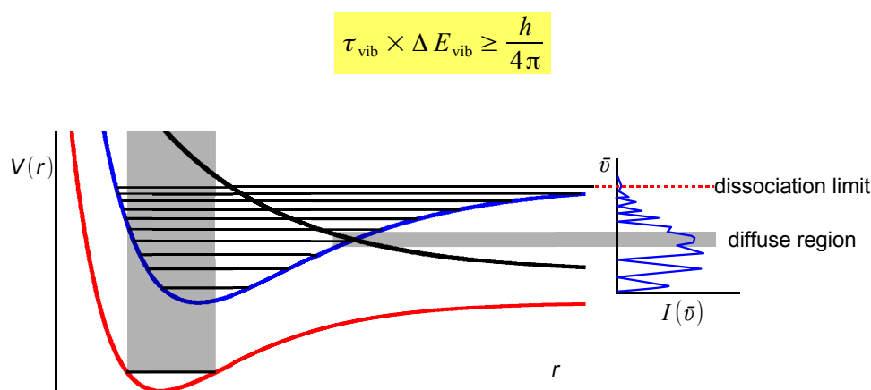
Figure 7.38: predissociation and diffuse spectra.
