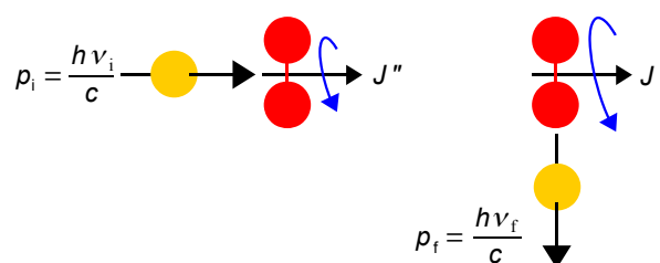
Figure 5.2: Stokes rotational Raman scattering viewed as a photon-molecule collision.
