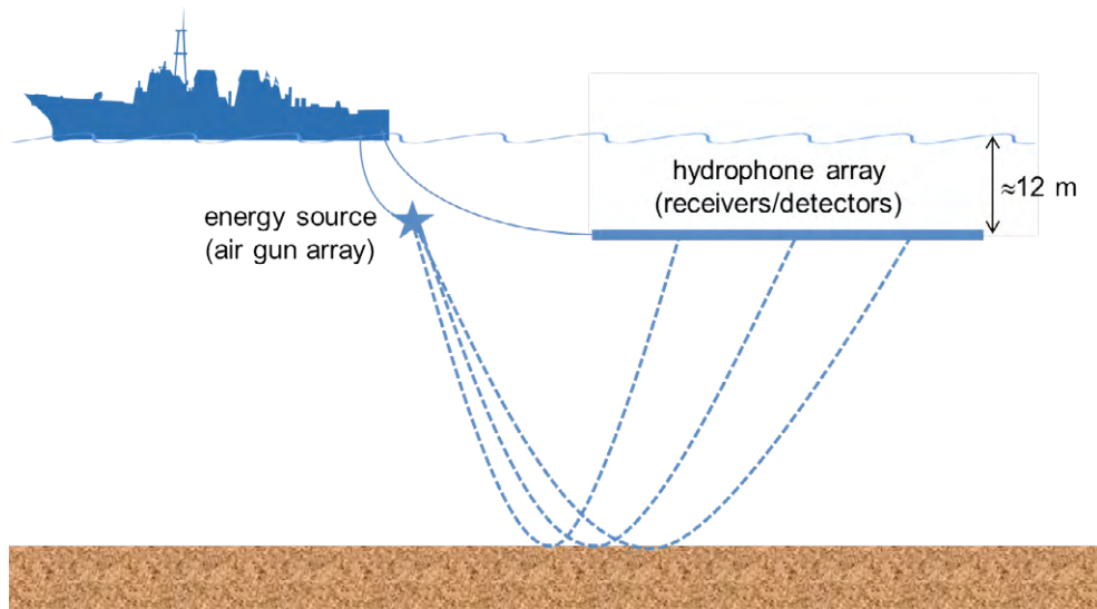
Figure 5-11. The use of sonar for the analysis of the ocean soil. During seismic surveys, high intensity, low frequency sounds are sent towards the earth's crust. They are reflected at different rates at certain geological boundaries. Analysis of the reflected sound informs the ship about the structure and composition of geological formations below the sea bed, as well as identify possible fossil fuel deposits.
