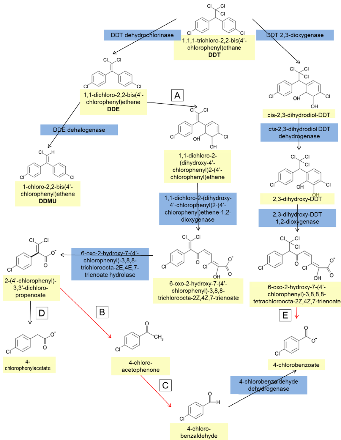
Figure 4-11. Aerobic breakdown of DDT with formation of different metabolites. Yellow boxes give compound names, blue boxes give the responsible enzymes. The steps labeled A, B, C, D, E are steps whose intermediates are not identified yet. Re arrows denote probable multistep reactions. (Taken from Gao et al. (2010), http://umbbd.ethz.ch/ddt/ddt_map.html ).
