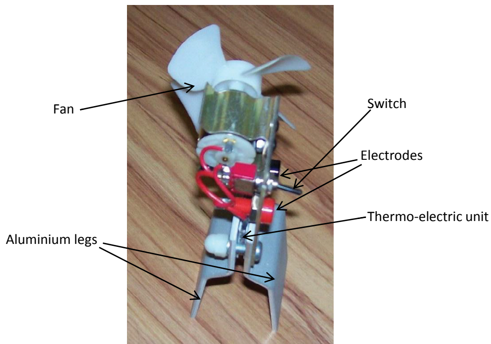
Figure 5.1: Thermo-electric device
