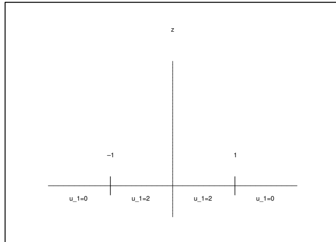
Figure 43: The Dirichlet problem of Figure 42 is by the map z_1 = \sin z mapped bijectively and conformally onto a simpler Dirichlet problem in the upper half z_1 -plane.
